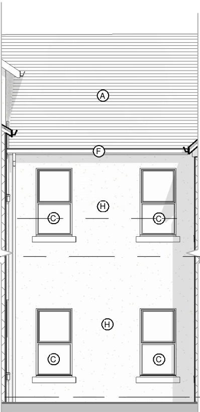
South Elevation1 : 100
