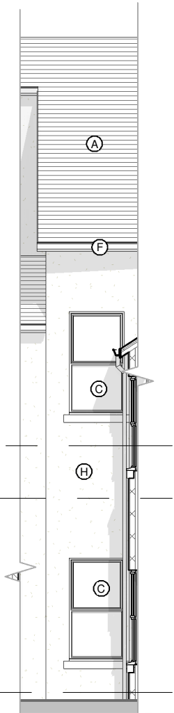
East Elevation1 : 100
