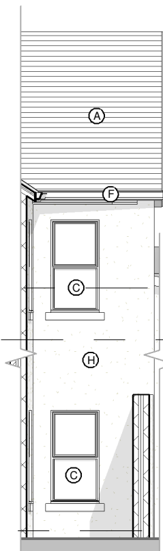
West Elevation1 : 100
