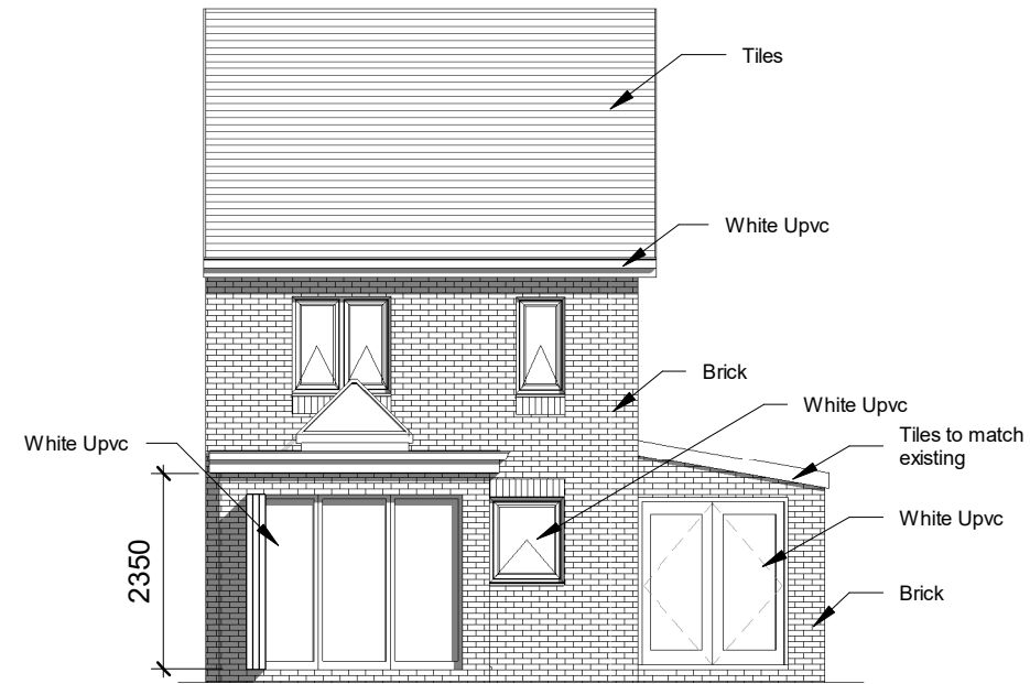
2 Proposed Rear Elevation 1 : 100
