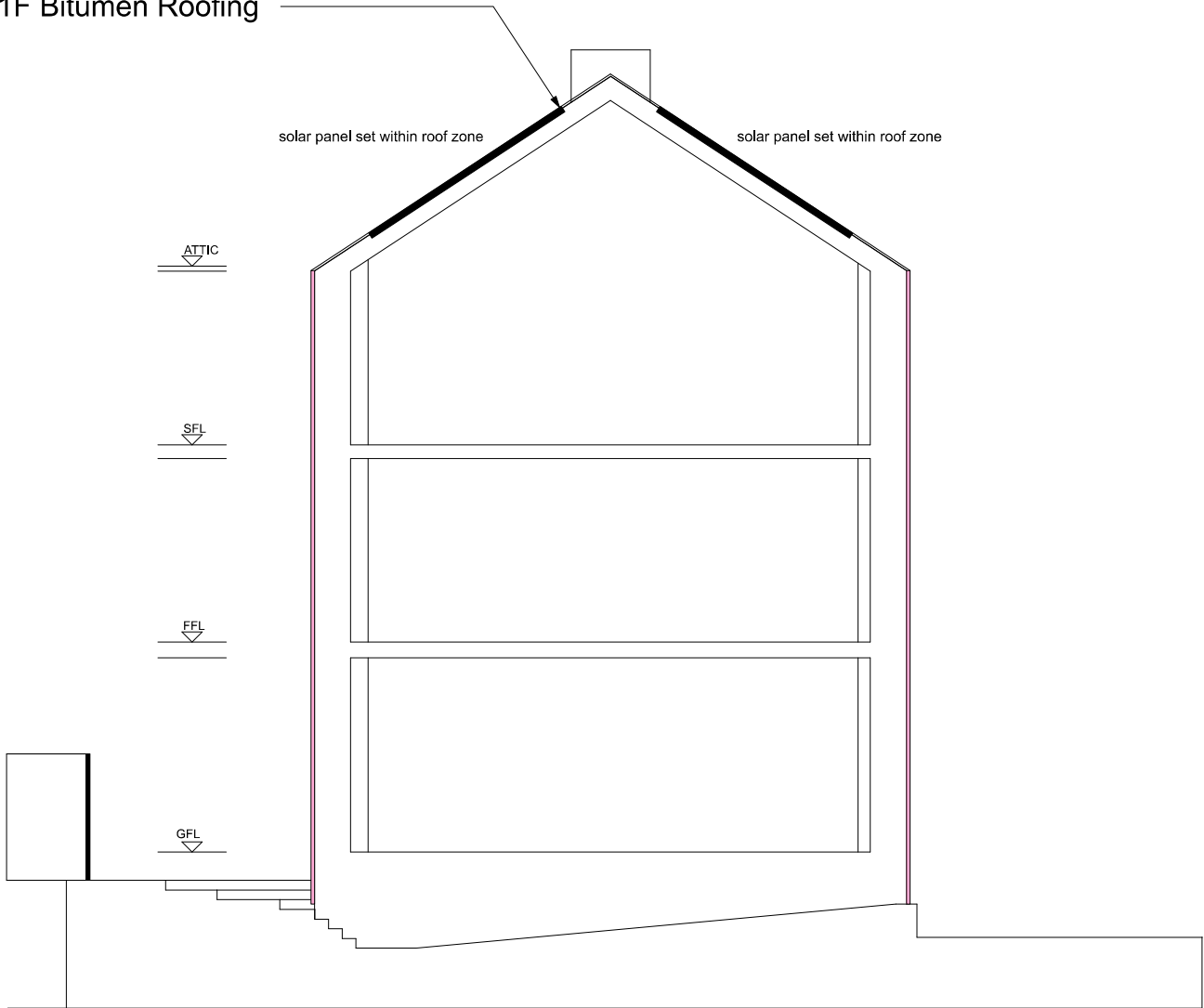
SECTION
