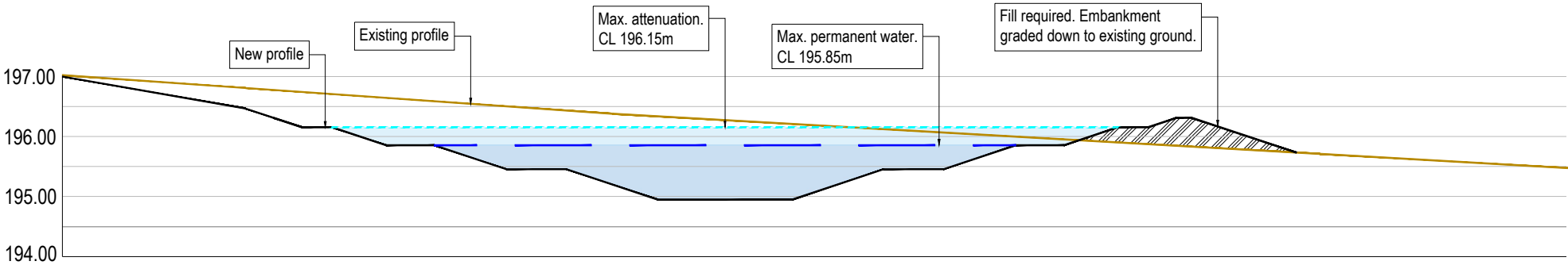
Section X-Y
