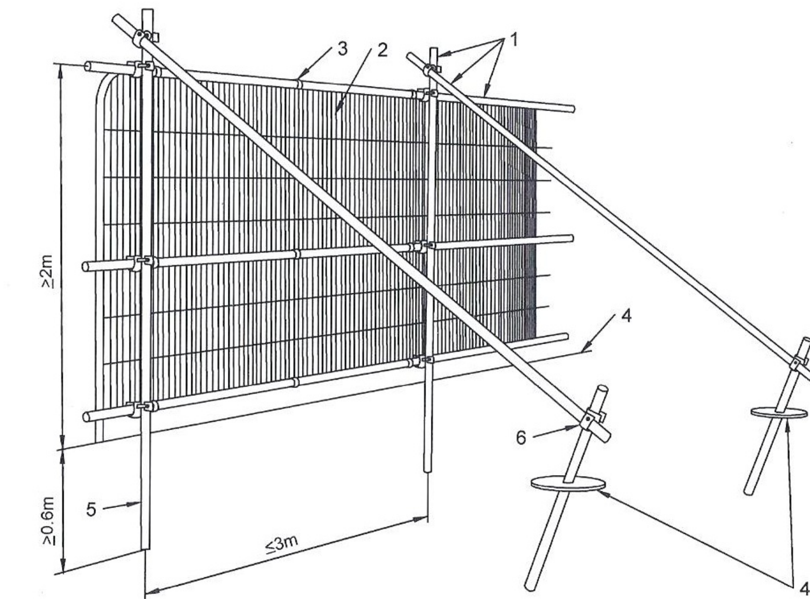
Figure 2 Default specification for protective barrier
