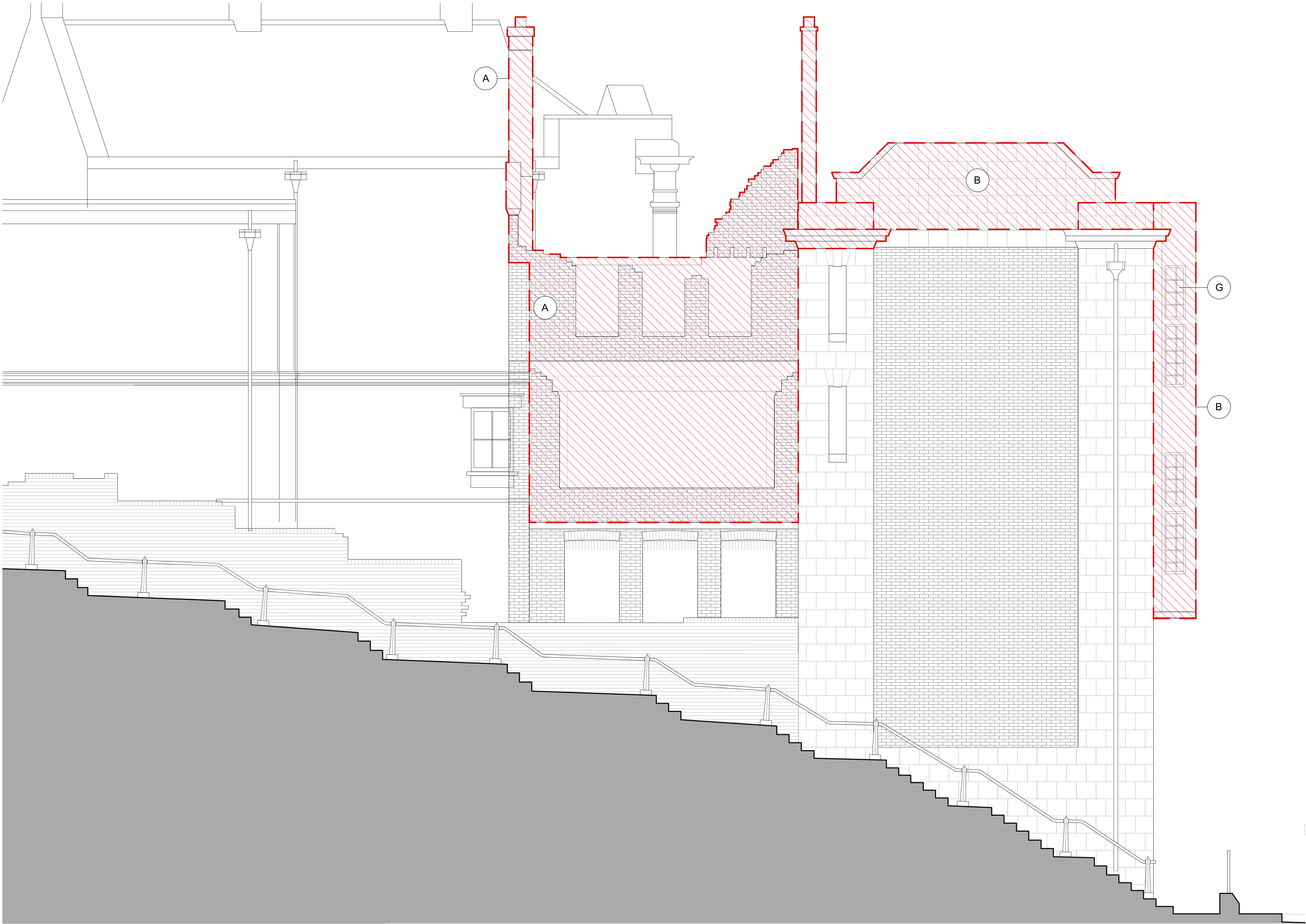
1 West Demolition Elevation Scale: 1:50
