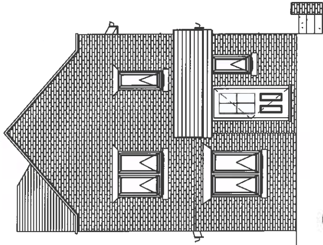
1 Proposed Front Elevation 1 : 100
