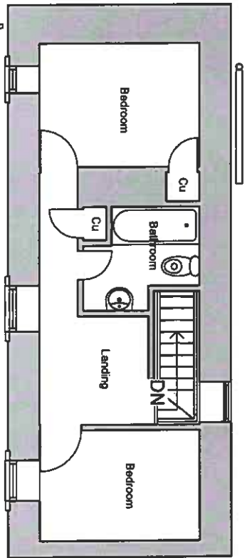
2 Existing First Floor 1 : 100
