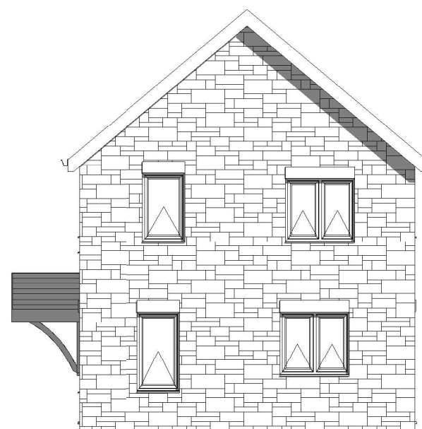
6 Side 2 Elevation 1 : 100
