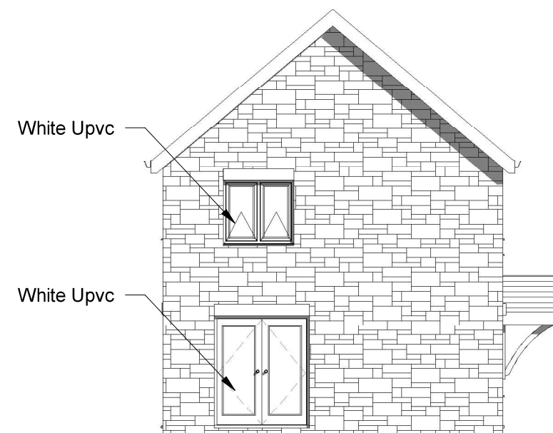
5 Side 1 Elevation 1 : 100
