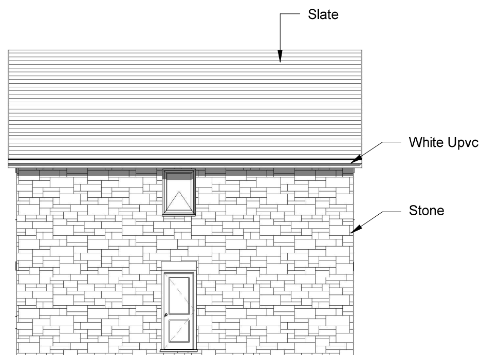
4 Rear Elevation 1 : 100
