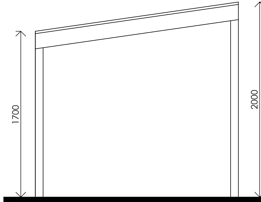
SIDE ELEVATION 1:20
