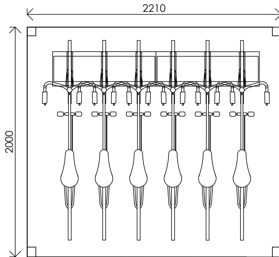
FRONT ELEVATION 1:20
