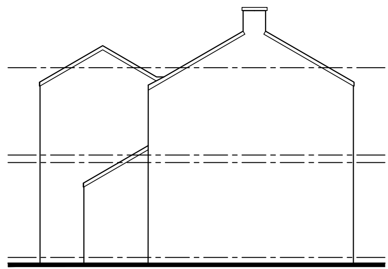
SIDE ELEVATION AS PROPOSED 1:100
