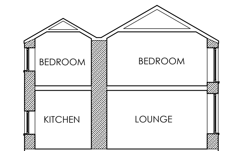
CROSS-SECTION AS EXISTING
