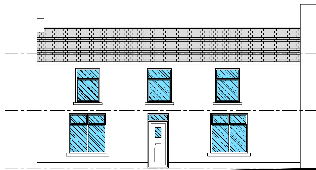
FRONT ELEVATION AS EXISTING
