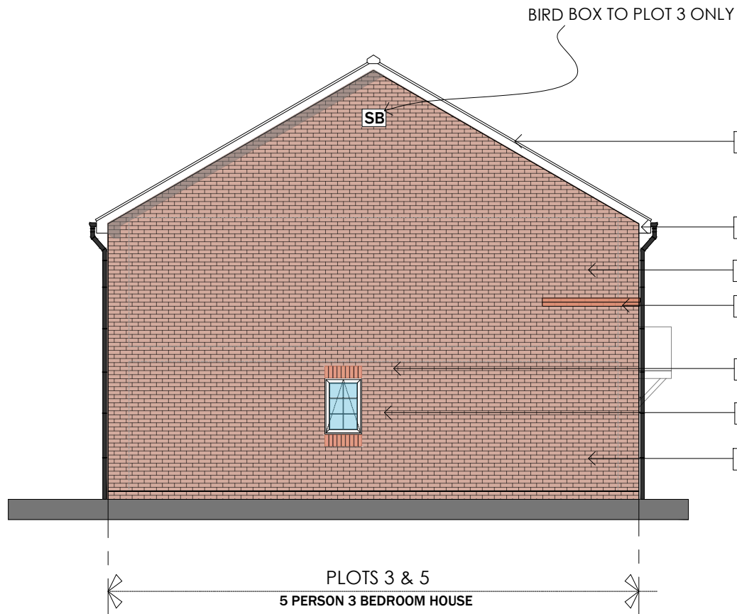
SIDE ELEVATION
