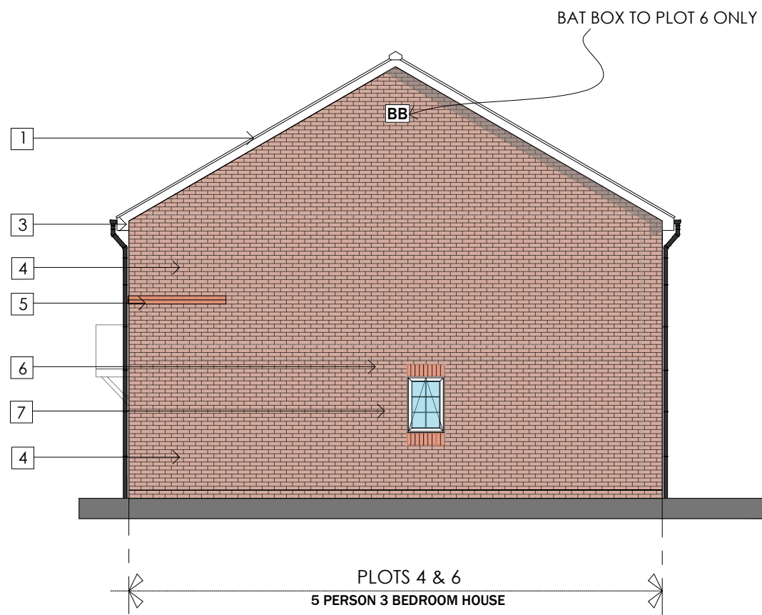
SIDE ELEVATION
