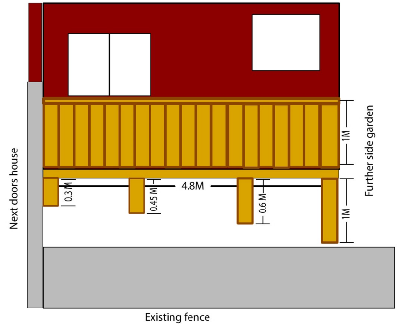
Front projection
