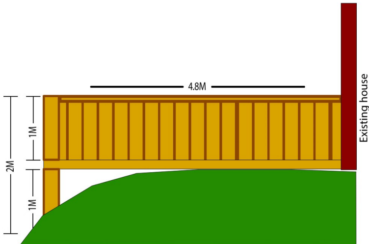
Side projection
