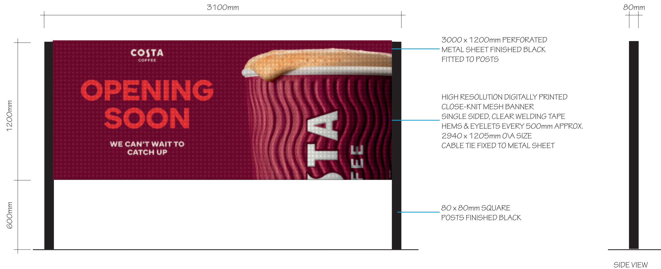
BANNER FRAME & MESH BANNER NON-ILLUMINATED Scale 1:20
