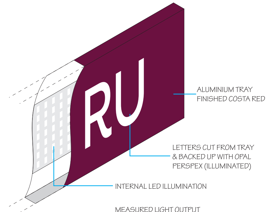
TRAY DETAIL
