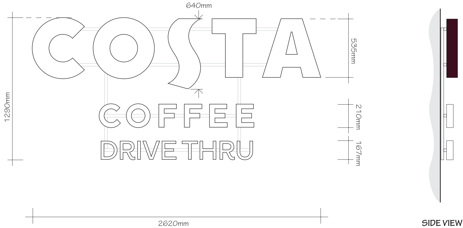
FRONT VIEW
