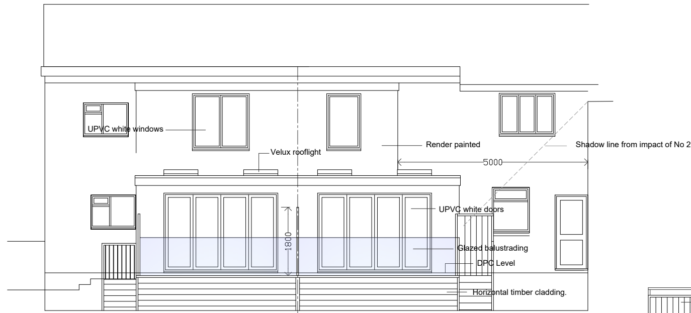
PROPOSED REAR ELEVATION (WEST)
