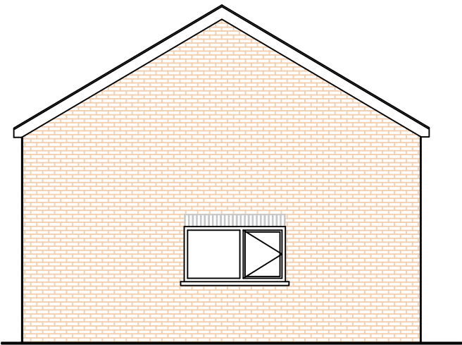
Proposed South East Facing Elevation
