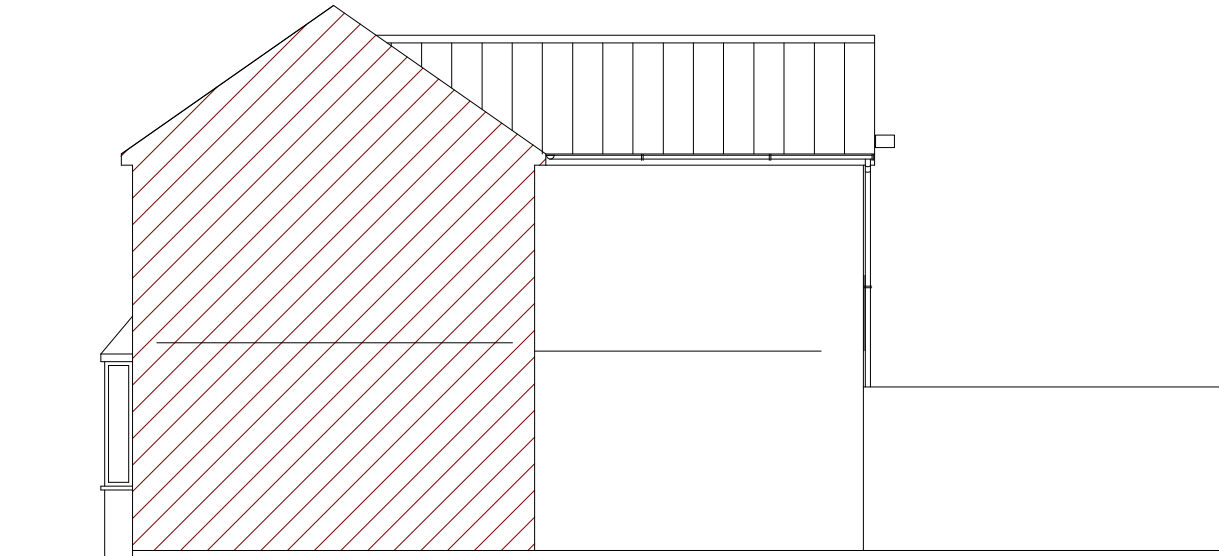
PROPOSED SIDE ELEVATION (viewed from No.39)
