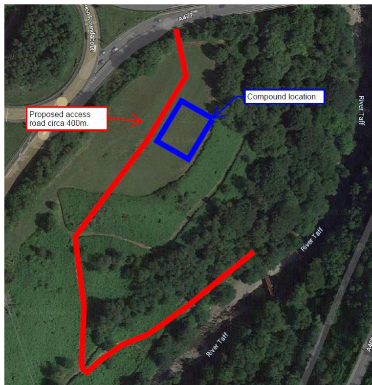
Figure 4 –Location of proposed access road and compound area
