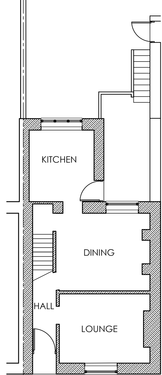
GROUND FLOOR PLAN AS EXISTING
