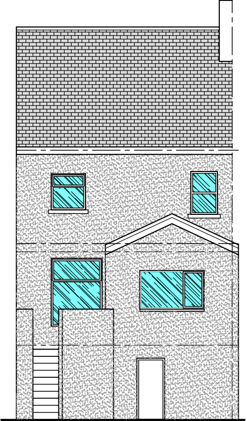
REAR ELEVATION AS EXISTING
