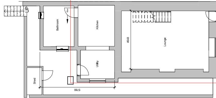
1 Existing Ground Floor. 1 : 100
