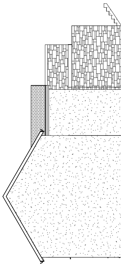
3 Existing Front Elevation. 1 : 100
