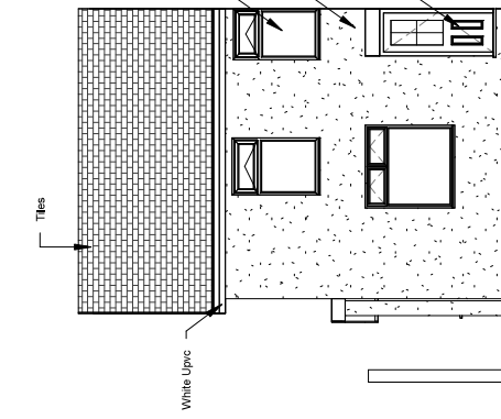
3 Existing Front Elevation. 1 : 100
