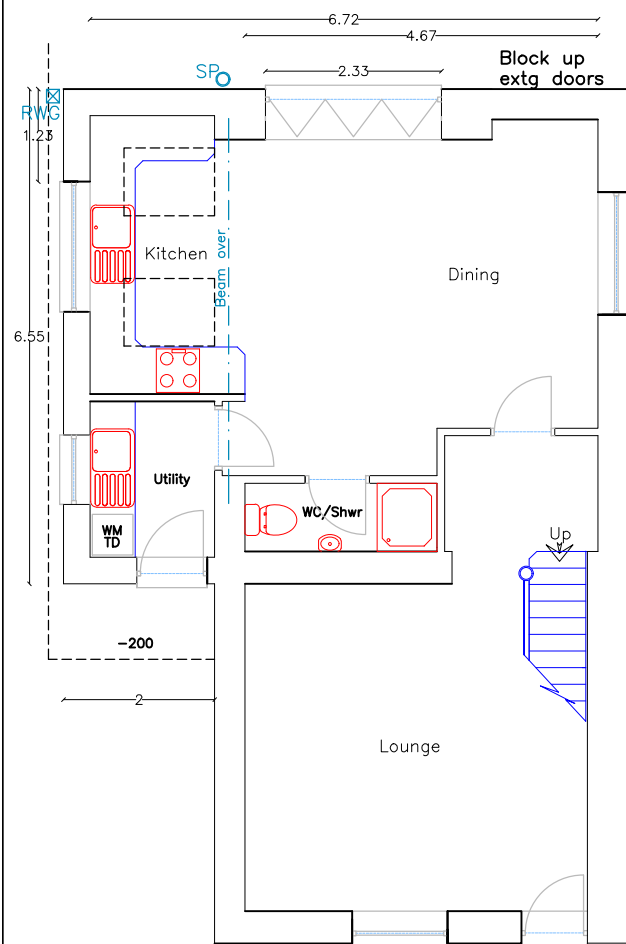
Proposed GF Plan 1:100
