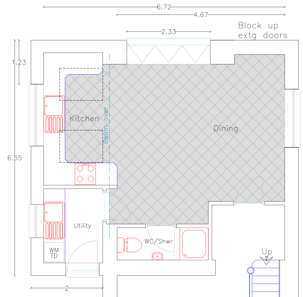
Proposed GF Plan 1:50
