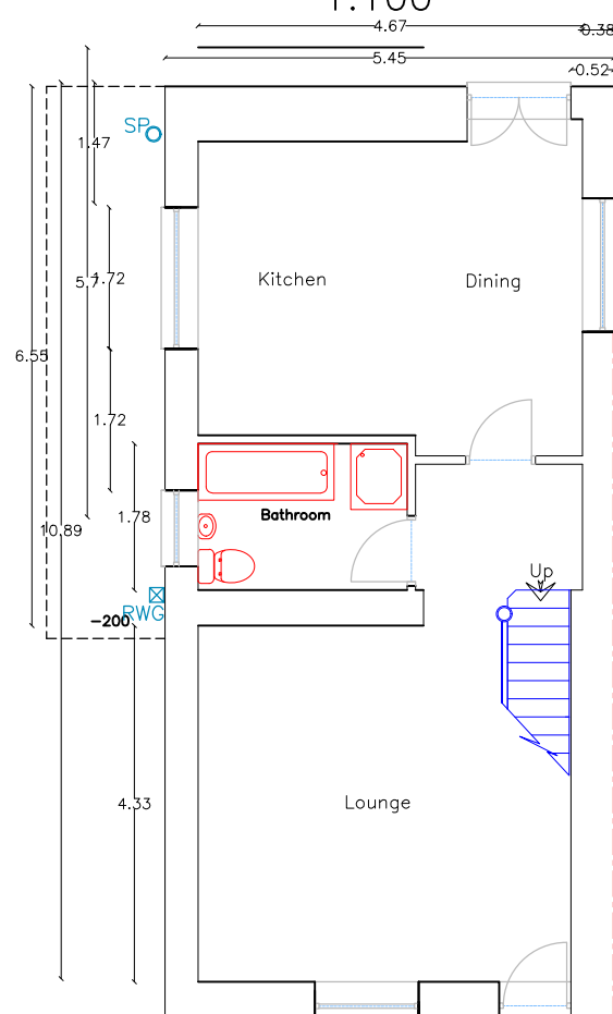
Existing GF Plan 1:100
