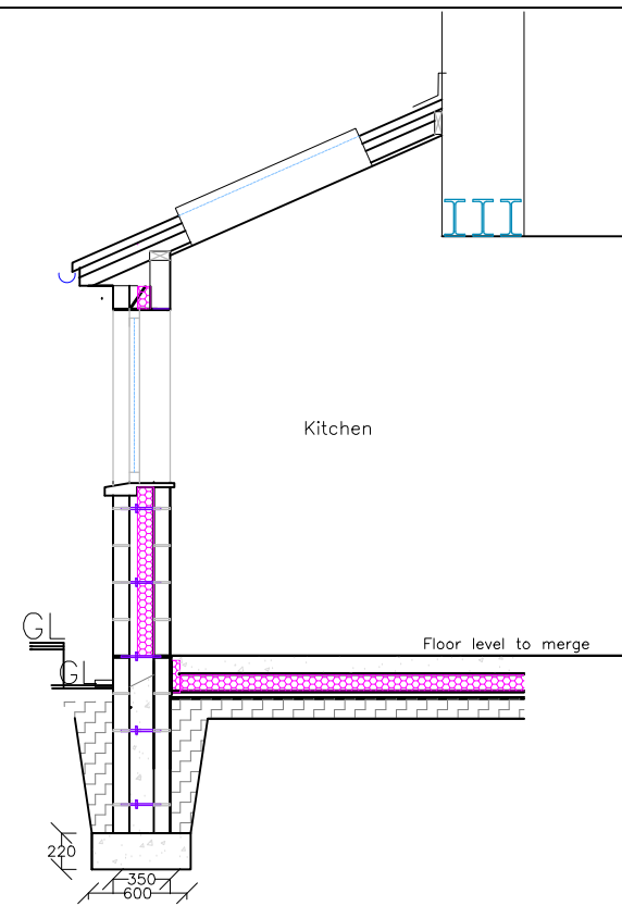
Proposed Section 1:50
