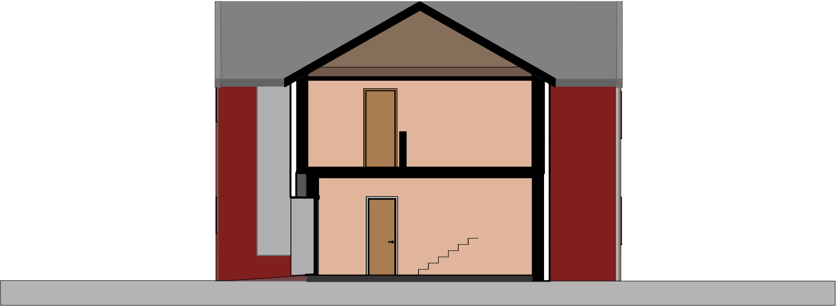
Section B-B
