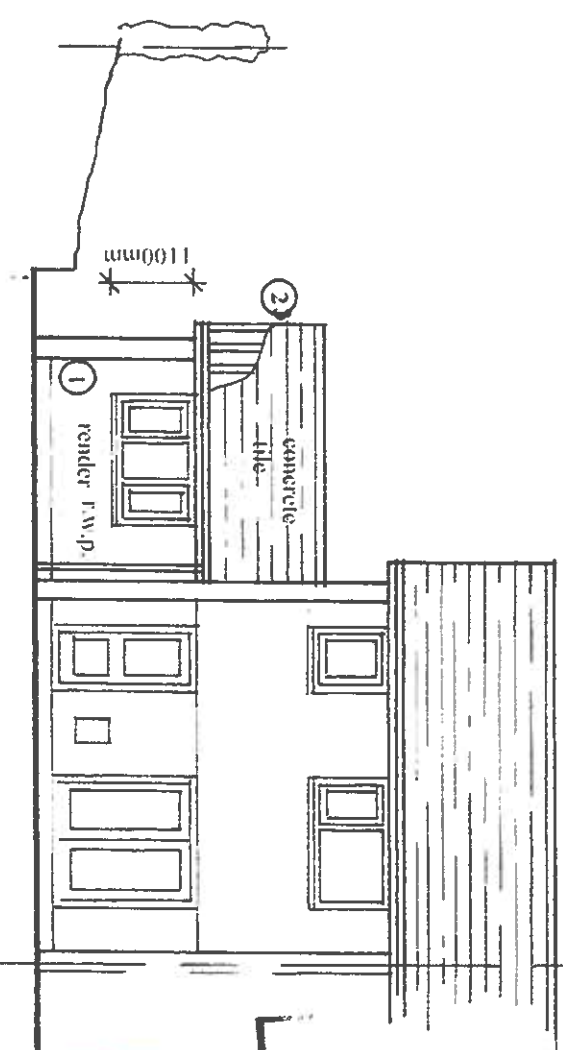
FRONT ELEVATION (1:100)
