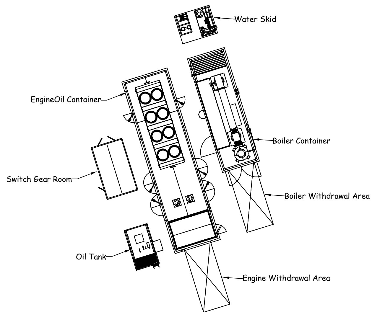
Floor Plan
