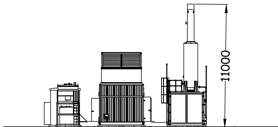
South Elevation
