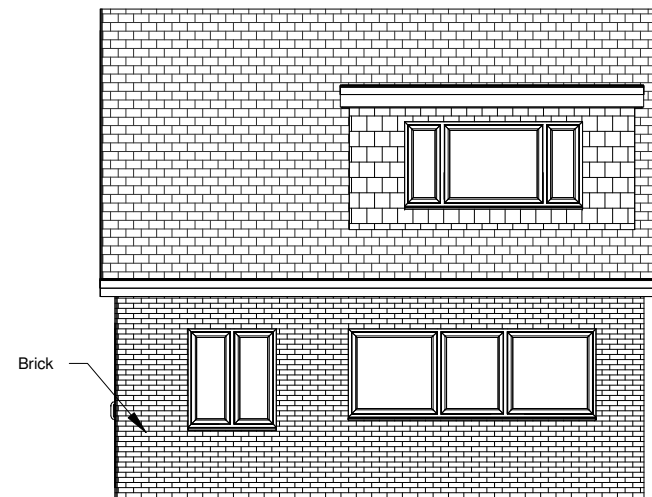
3 Existing Front Elevation 1 : 100
