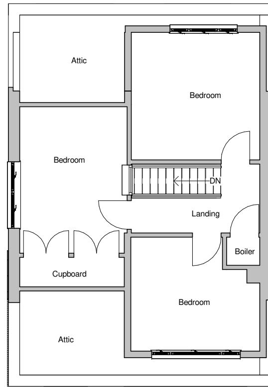
2 Existing First Floor 1 : 100
