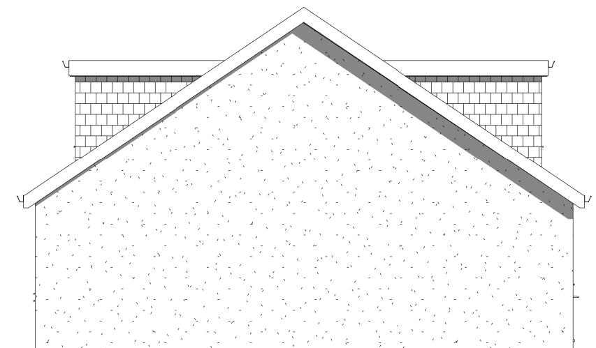
6 Existing Side 2 Elevation 1 : 100
