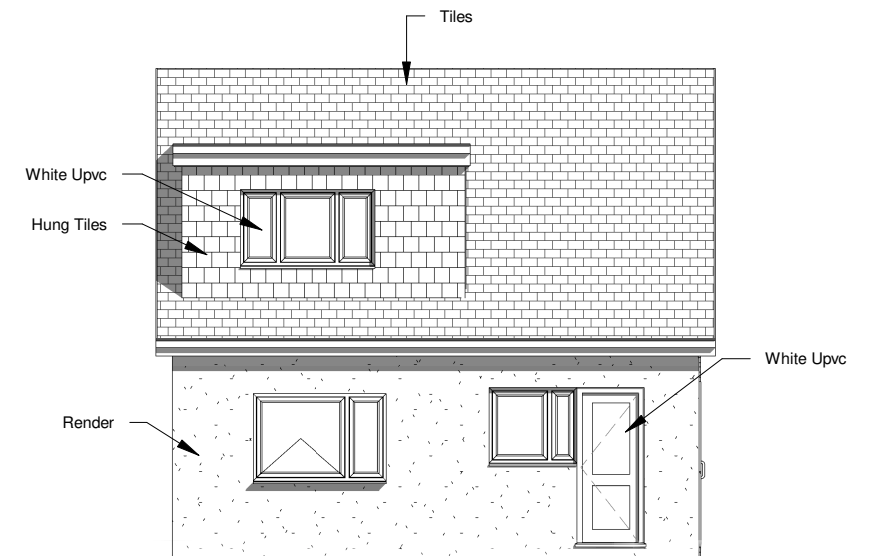
4 Existing Rear Elevation 1 : 100
