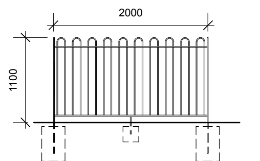
HOOP TOP RAILINGS 1:50
