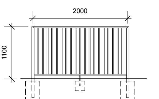
RAILINGS TO MATCH EXISTING 1:50
