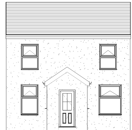
1 Proposed Front Elevation 1 : 100
