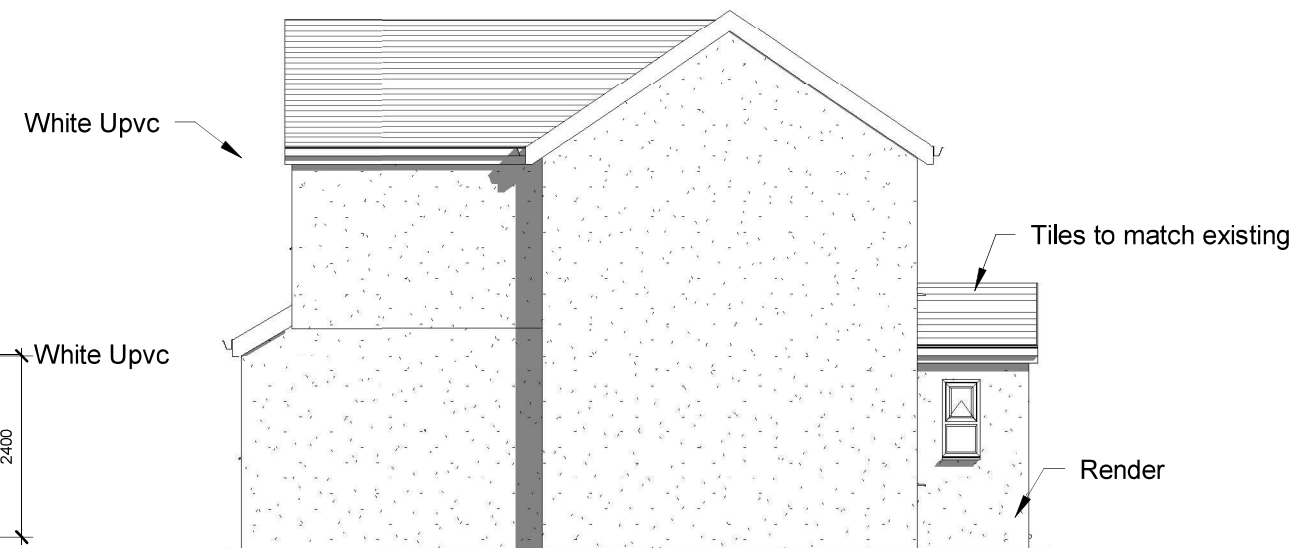
3 Proposed Side 1 Elevation 1 : 100
