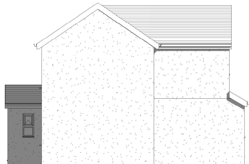
4 Proposed Side 2 Elevation 1 : 100
