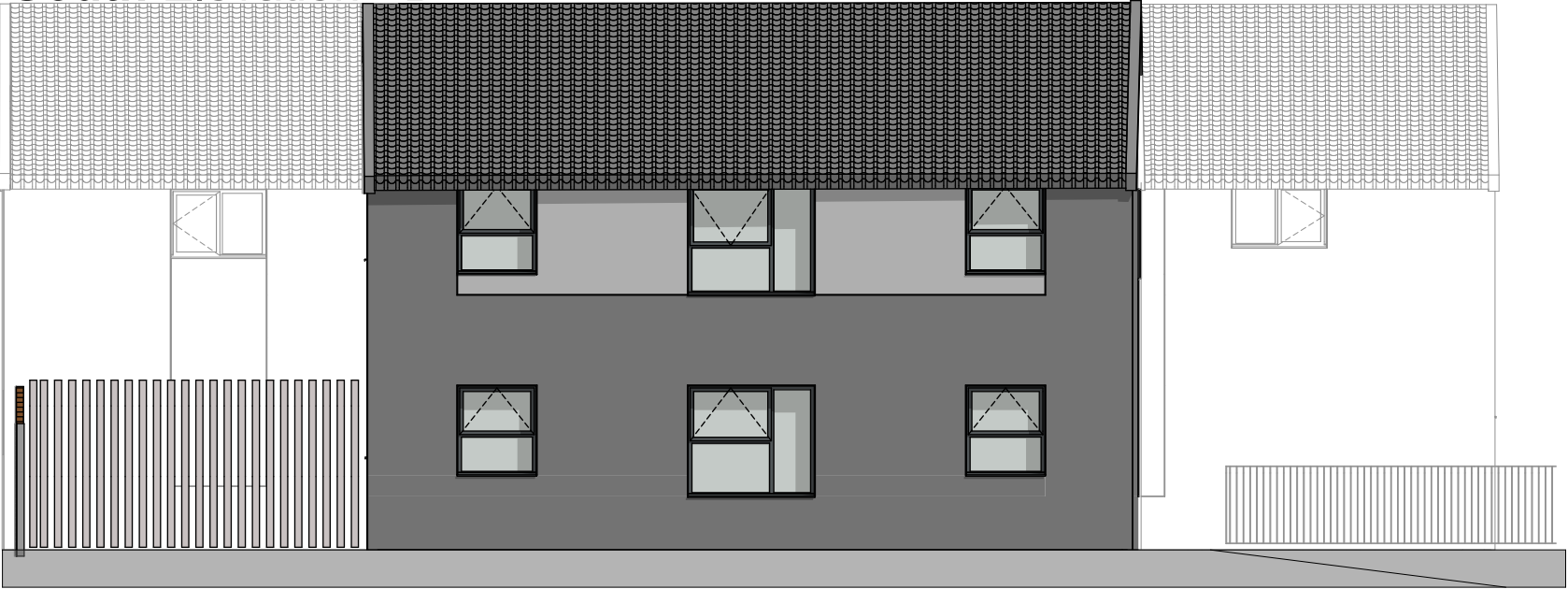
North Elevation - B
