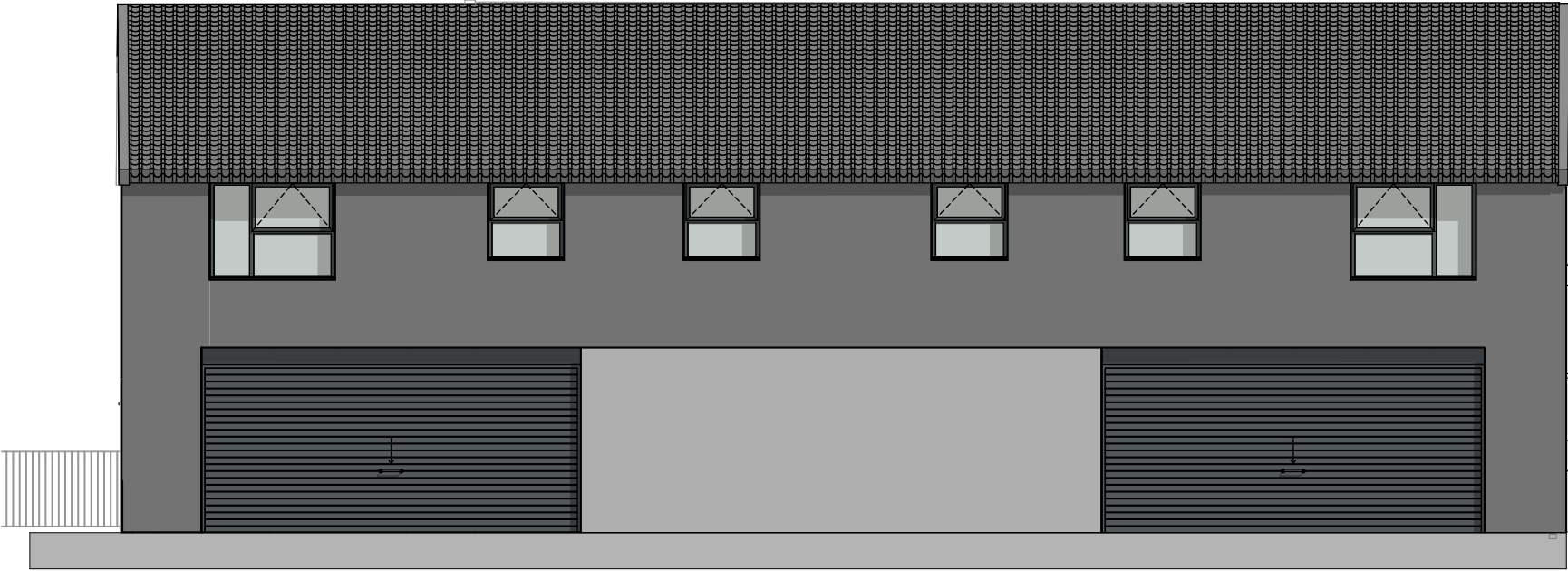
South Elevation - D
