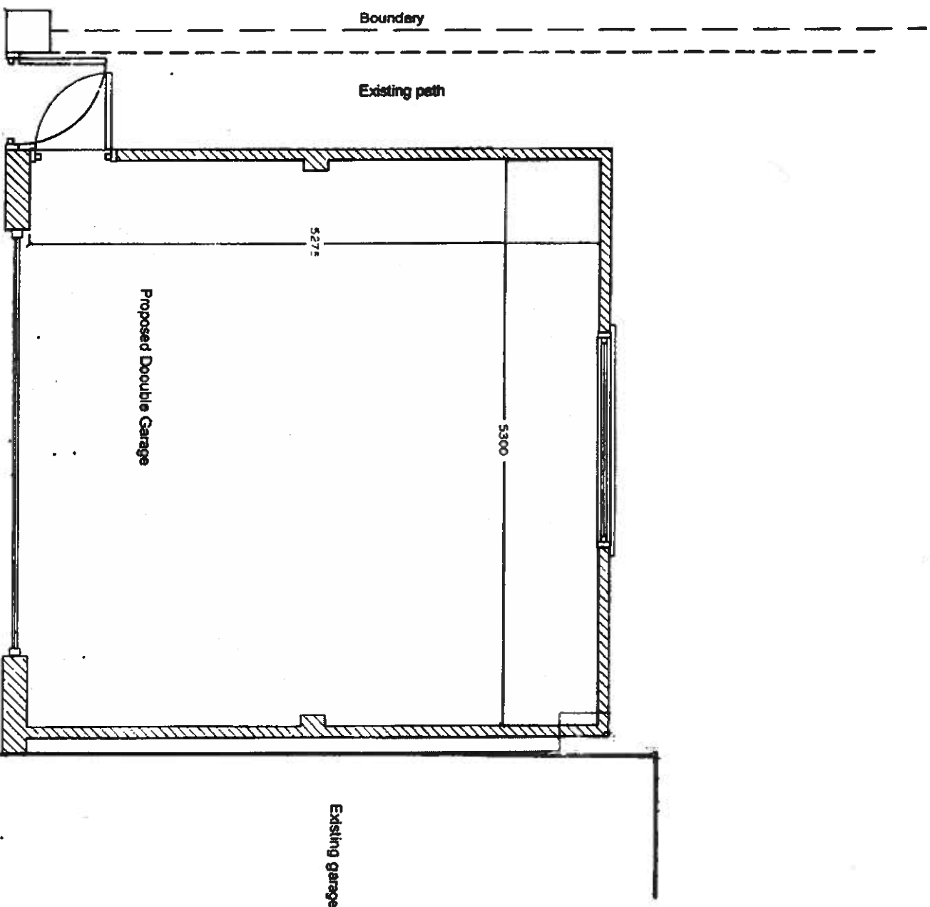
PROPOSED PLAN (1:50)
