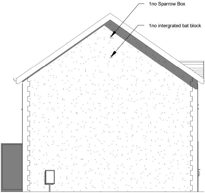
5 Side 1 Elevation 1 : 100
