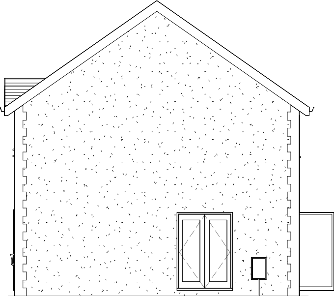
6 Side 2 Elevation 1 : 100
