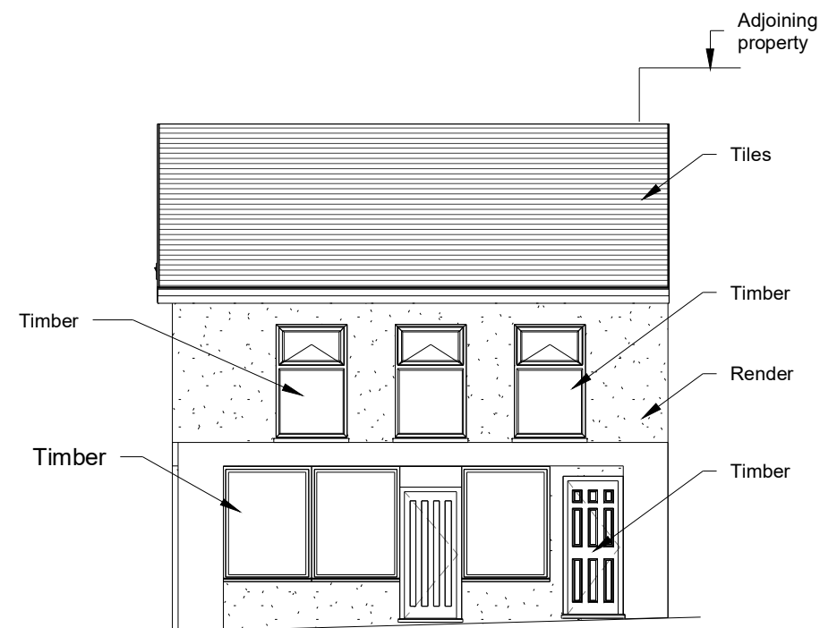
1 Existing Front Elevation 1 : 100
