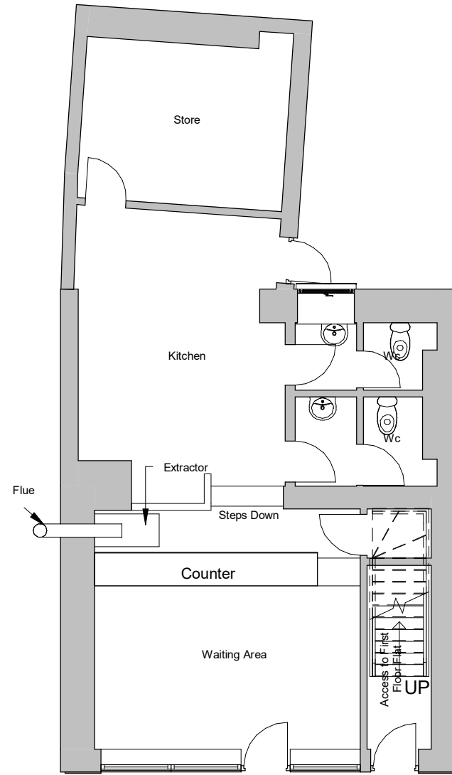
1 Proposed Ground Floor 1 : 100
