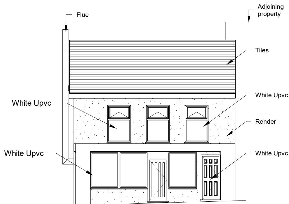
1 Proposed Front Elevation 1 : 100
