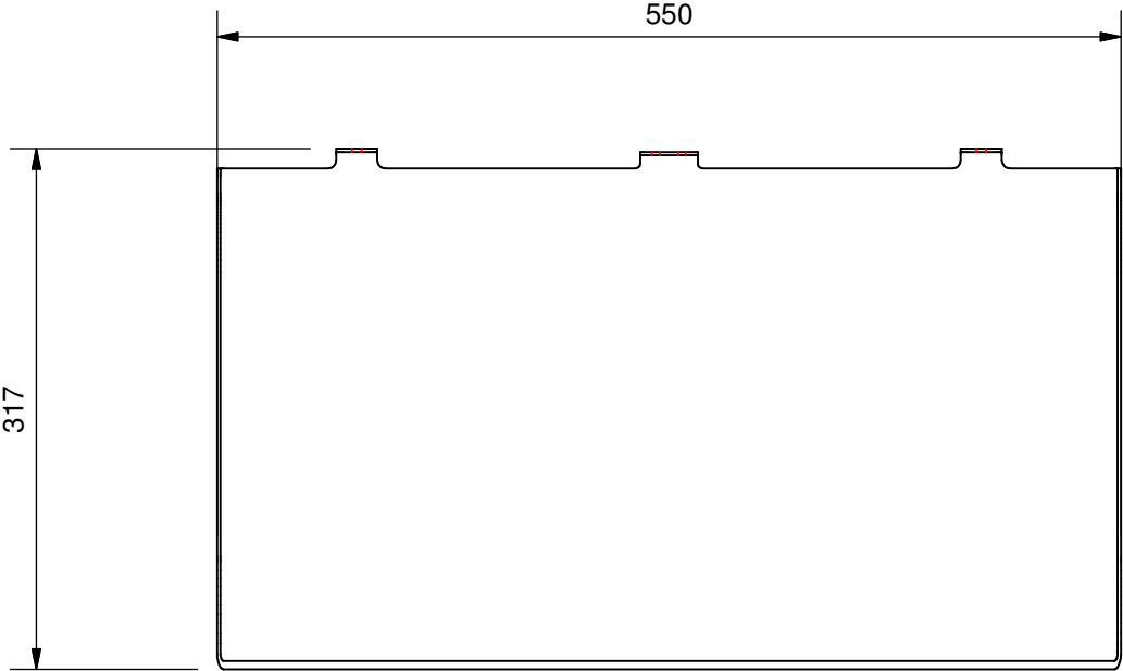
FRONT (SCALE 1 : 5 )
