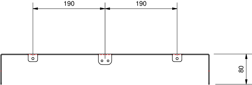
PLAN (SCALE 1 : 5 )
