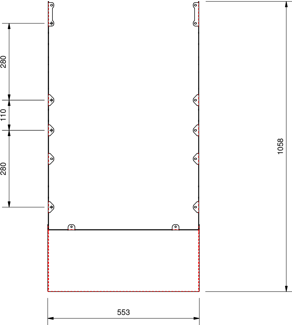
PLAN (SCALE 1 : 8 )
