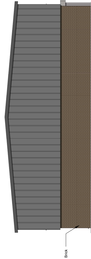
1 Existing Side 2 Elevation 1 : 100
