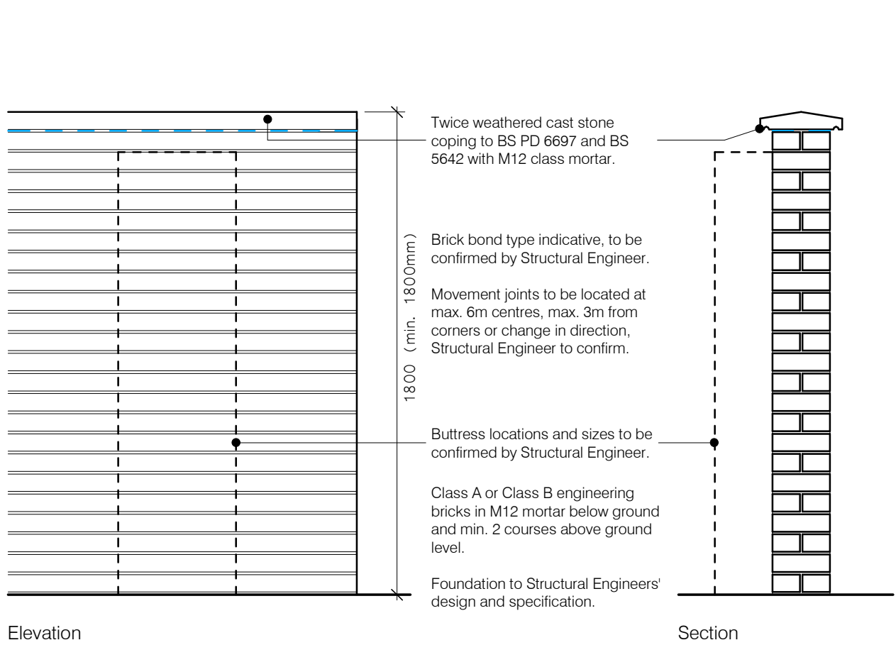
Boundary Type 1 - - - - - 1800mm high facing brickwork walls with cast stone coping.
