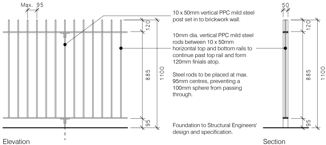
Boundary Type 6 - - - - - 1100mm high PPC metal bar railings.
