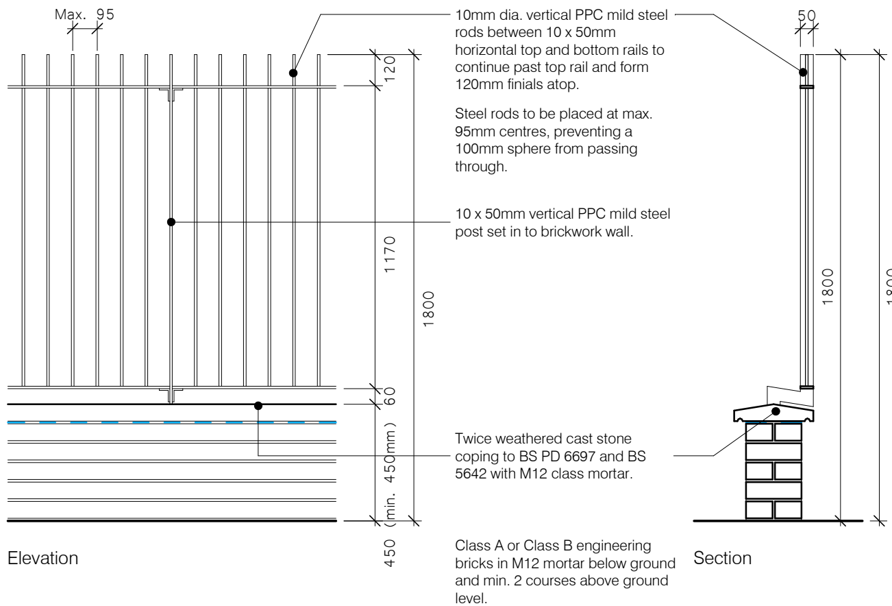
Boundary Type 4 - - - - - 450mm high facing brickwork walls with cast stone coping and PPC metal bar railings atop up to 1800mm.
