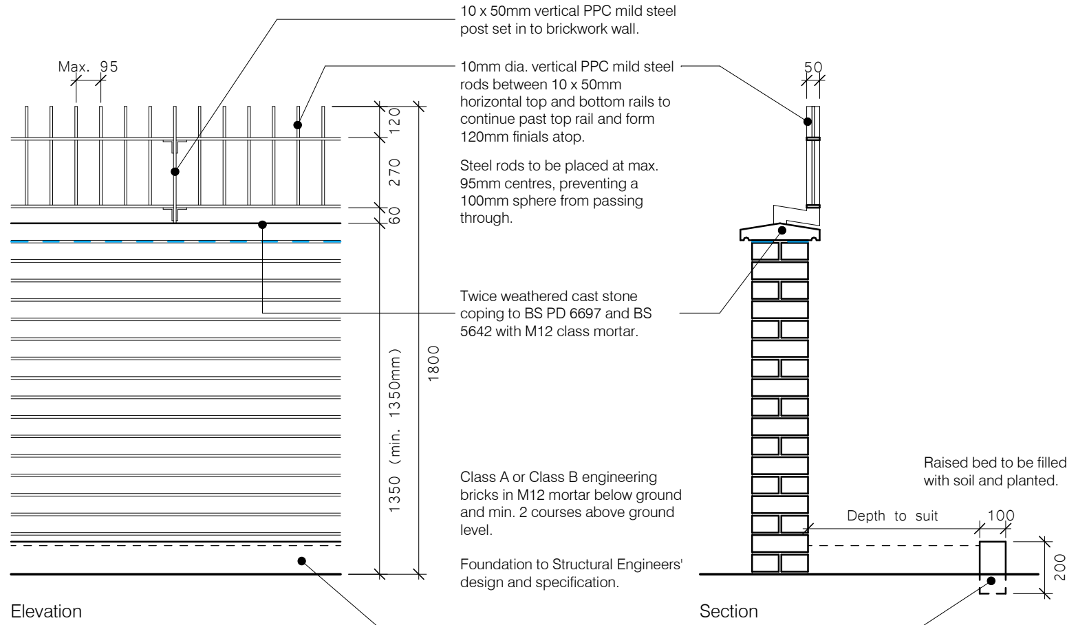
Boundary Type 3 - - - - - 1350mm high facing brickwork walls with cast stone coping and PPC metal bar railings atop up to 1800mm. Planting bed to front.
