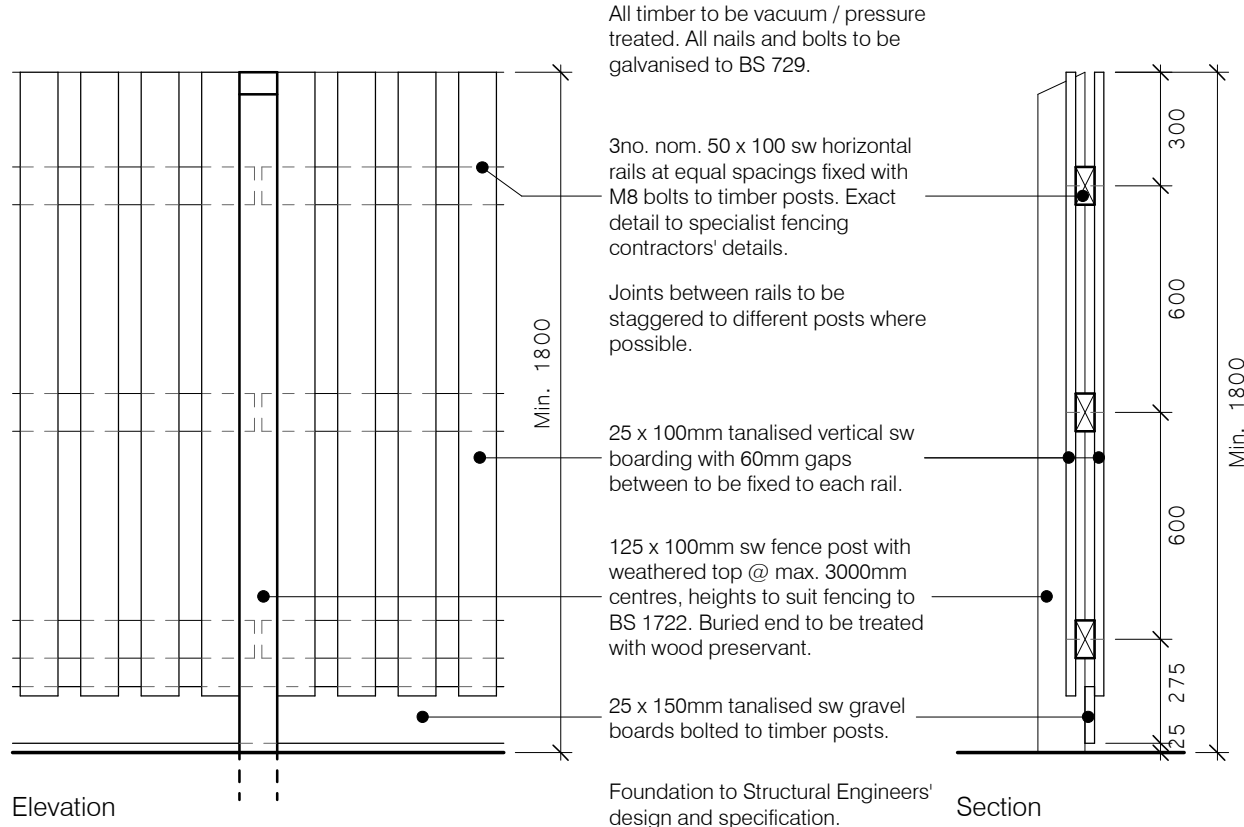
Boundary Type 5 - - - - - 1800mm high double sided hit & miss timber fencing (single side where indicated).
