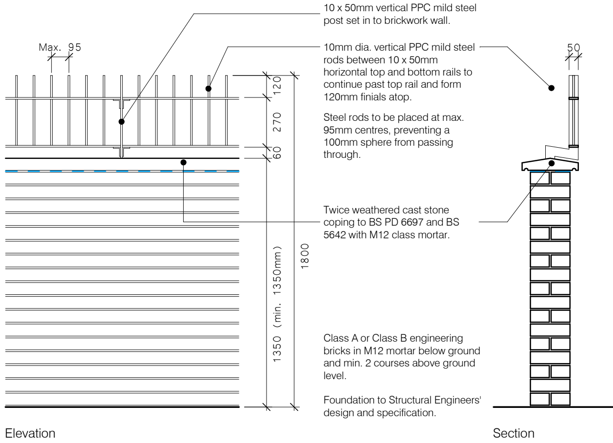
Boundary Type 2 - - - - - 1350mm high facing brickwork walls with cast stone coping and PPC metal bar railings atop up to 1800mm.
