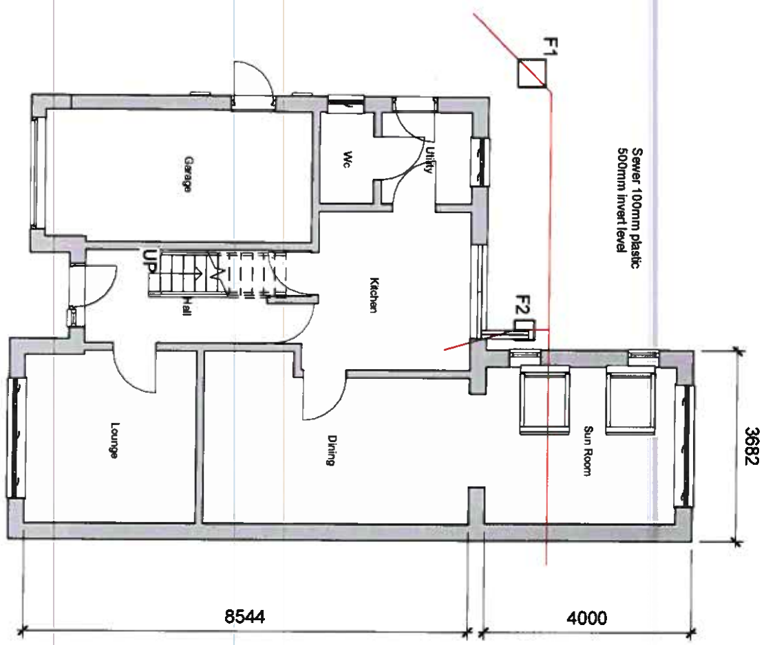
1 Proposed Ground Floor 1 : 100
