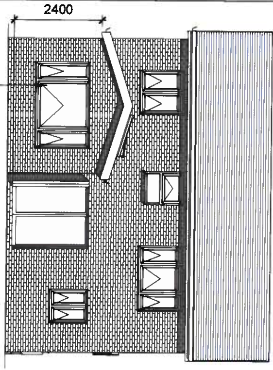
4 Proposed Rear Elevation 1 : 100
