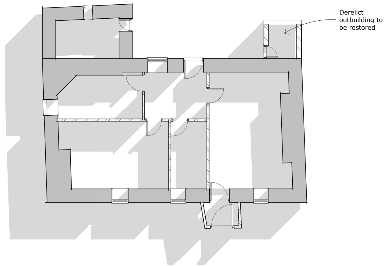
5 Existing Ground Floor Plan 1 : 100
