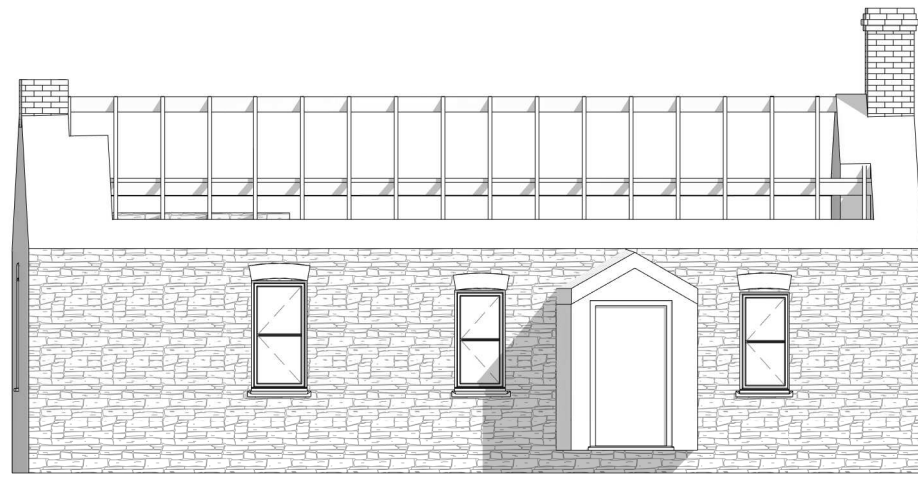
1 Existing South West 1 : 100
