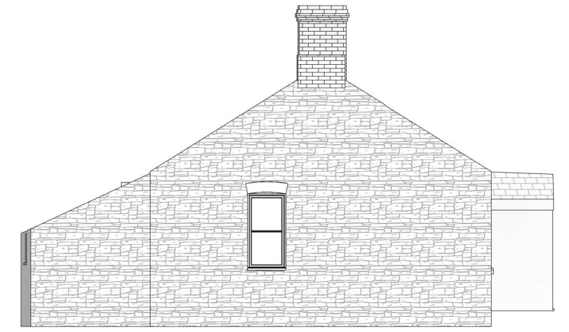
3 Existing North West 1 : 100
