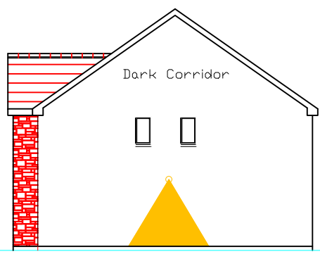
SIDE ELEVATION
