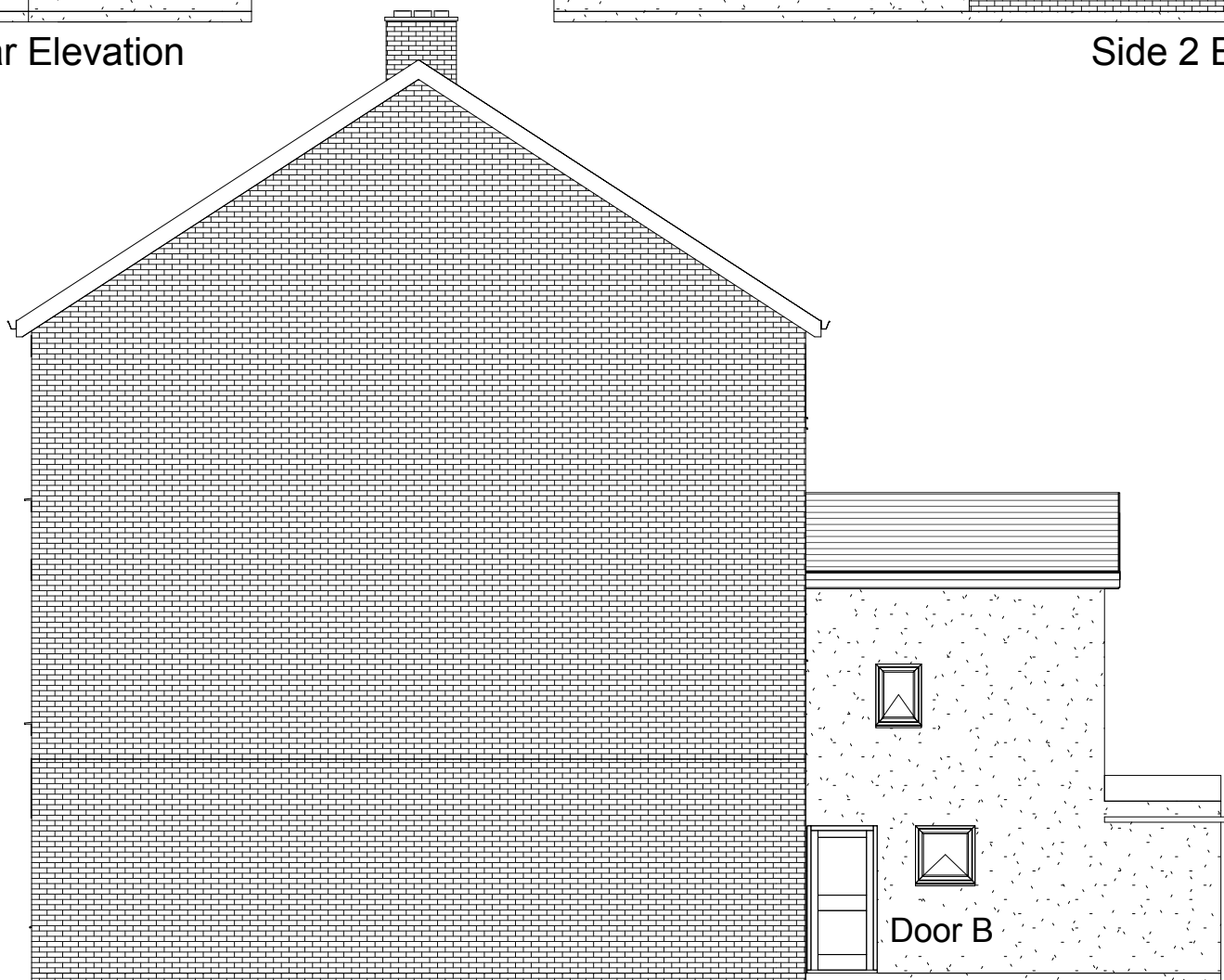
Side 1 Elevation
