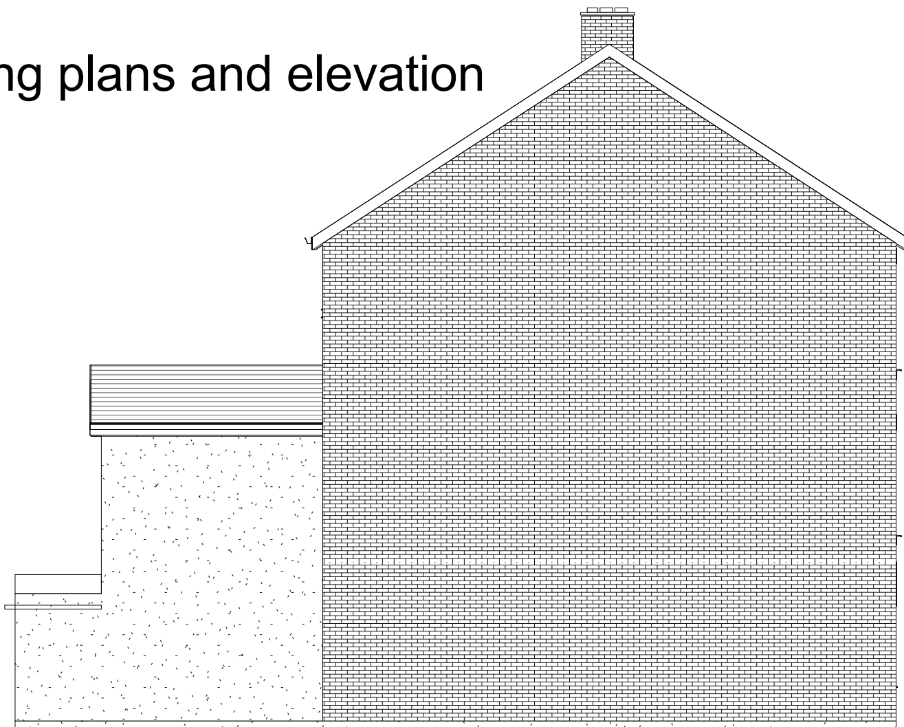
Side 2 Elevation
