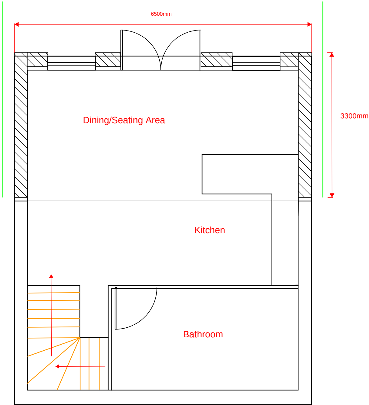
Proposed Lower Ground Floor Plan - 1:50
