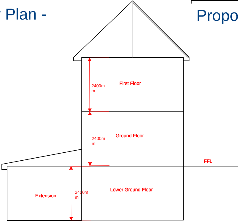
Proposed Section Through/Side Elevation View - 1:100
