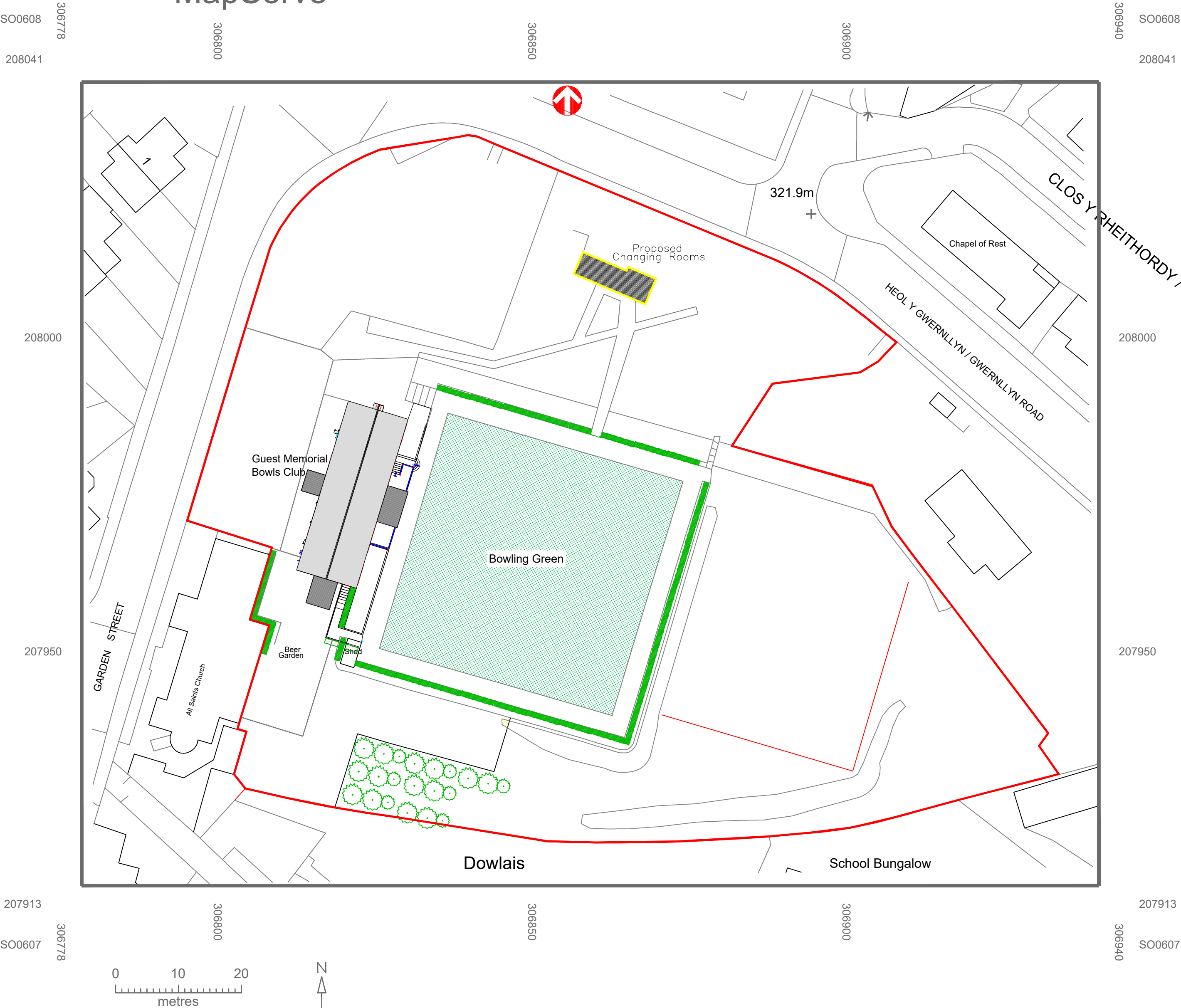
Location Plan 1:500
