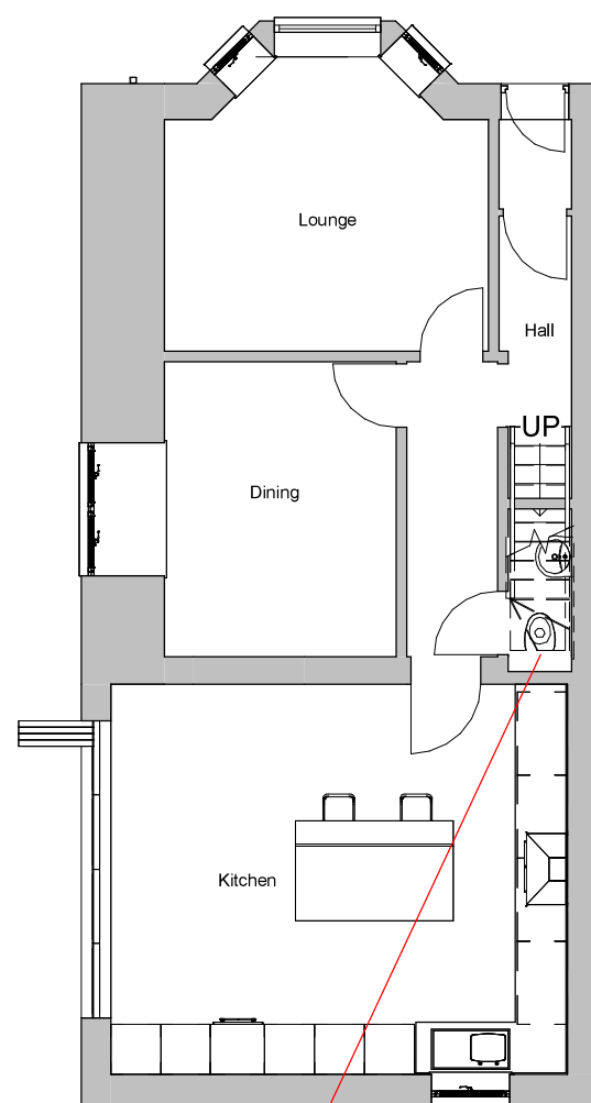
1 Proposed Ground Floor 1 : 100
