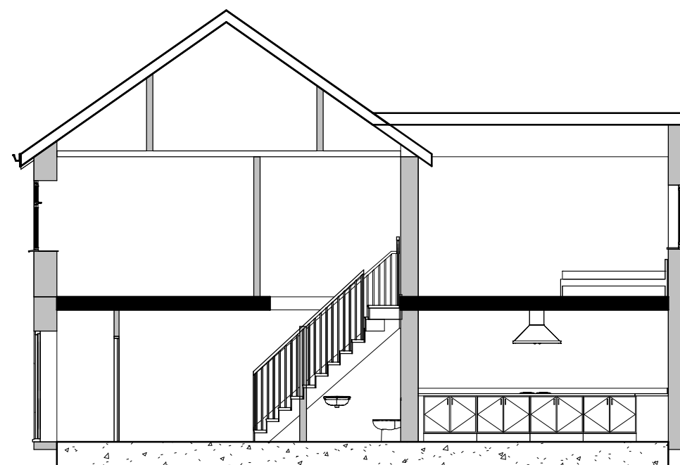
4 Proposed Section 1 : 100
