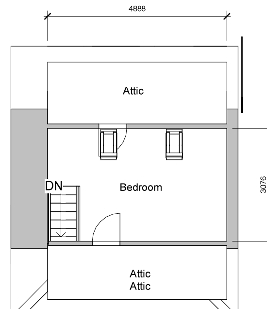
3 Proposed Second Floor 1 : 100
