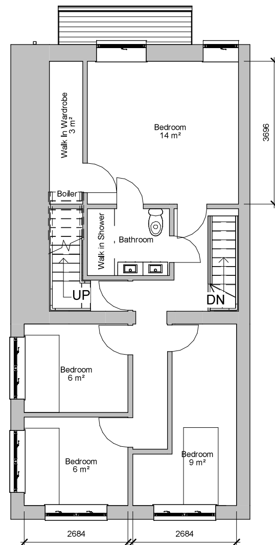
2 Proposed First Floor 1 : 100
