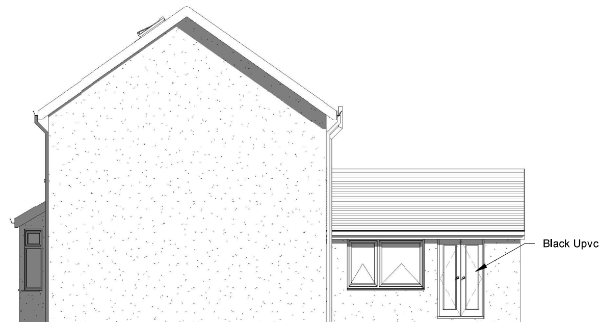
3 Existing Side 1 Elevation 1 : 100
