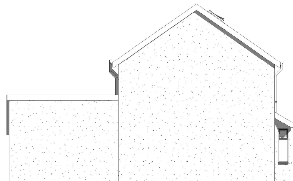
4 Existing Side 2 Elevation 1 : 100
