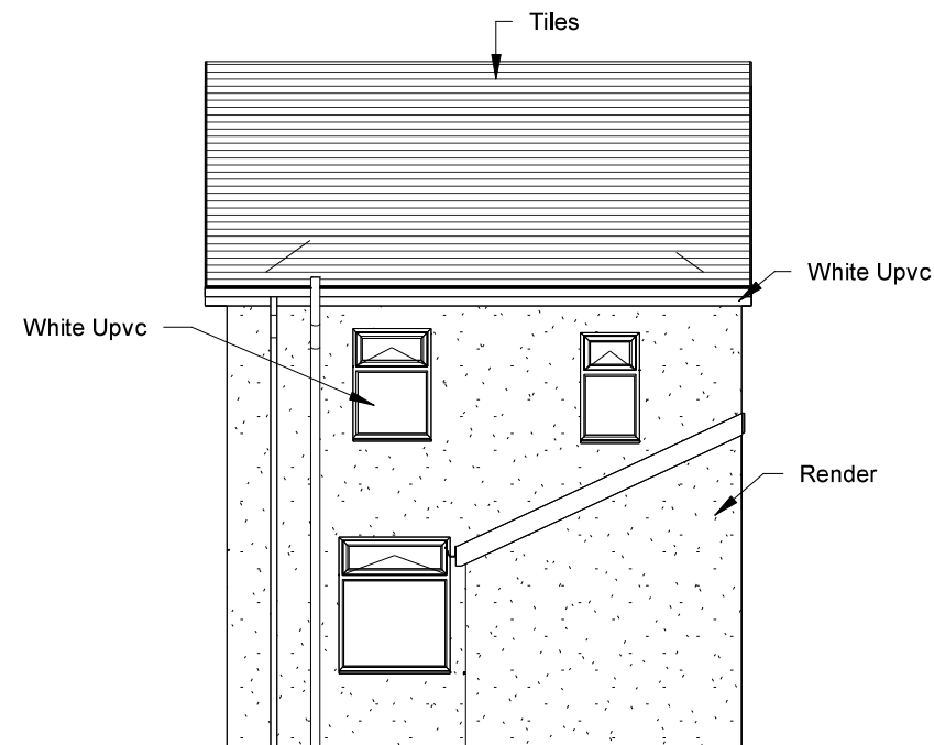
2 Existing Rear Elevation 1 : 100
