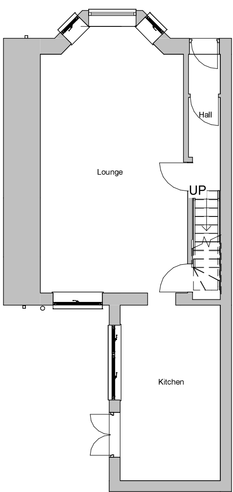
1 Existing Ground Floor 1 : 100
