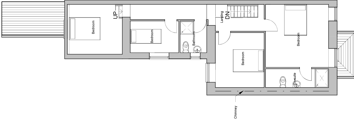
2 Proposed First Floor 1 : 100
