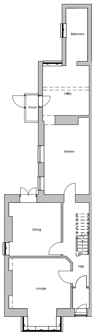
1 Existing Ground Floor 1 : 100
