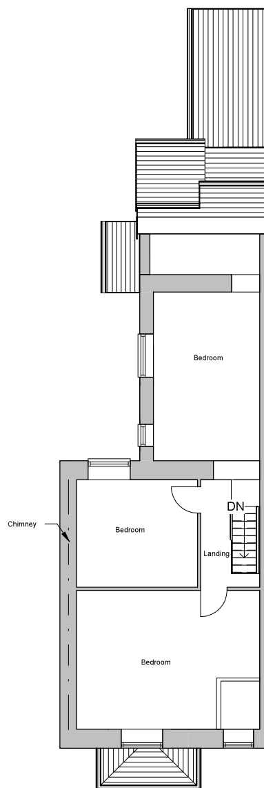
2 Existing First Floor 1 : 100
