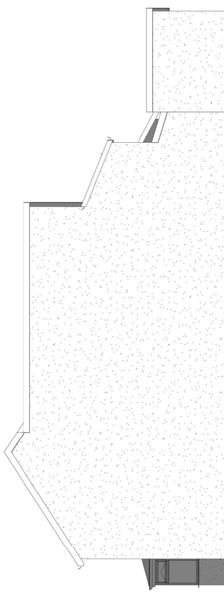
4 Existing Side 2 Elevation 1 : 100
